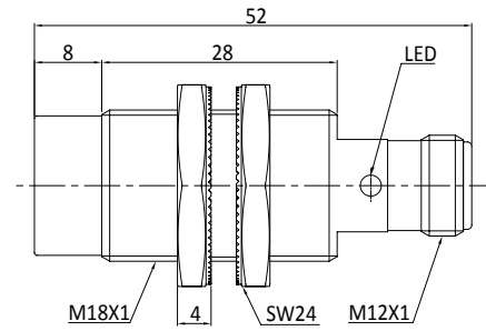
Fig. 8 Inductive sensor with M12 connector (non-flush)
