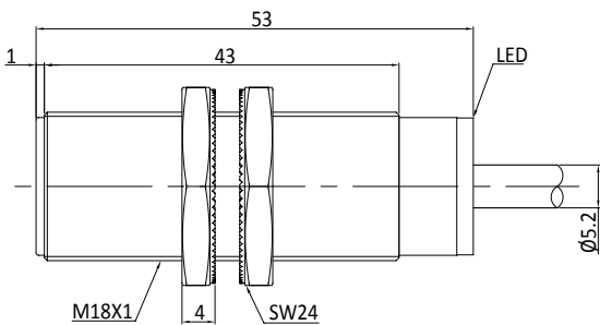
Fig. 5 Inductive sensor with cable (flush)
