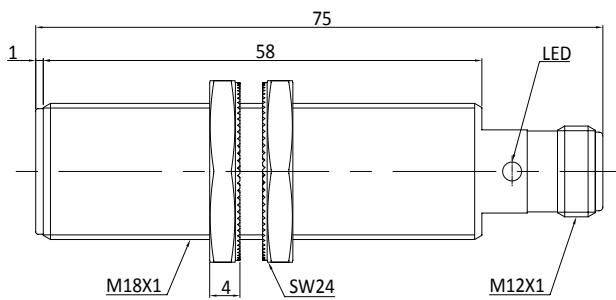
Fig. 9 Inductive sensor with M12 connector (flush)
