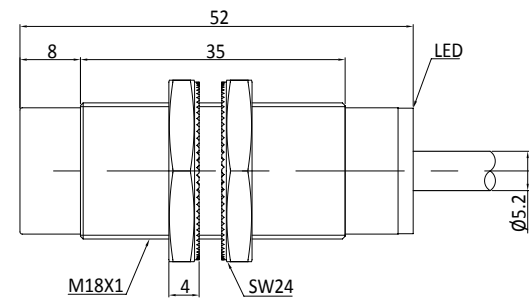
Fig. 6 Inductive sensor with cable (non-flush)
