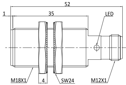
Fig. 7 Inductive sensor with M12 connector (flush)
