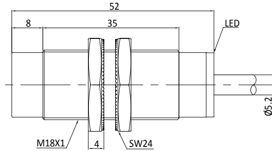
Fig. 2 Inductive sensor with cable (non-flush)
