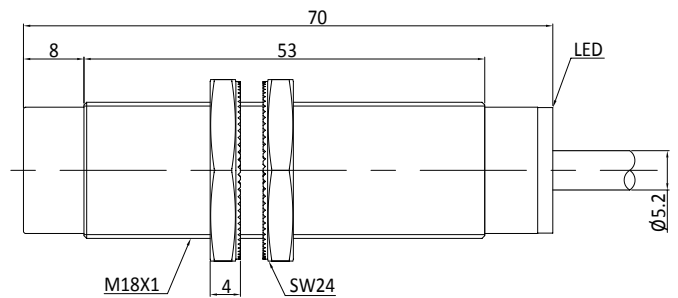
Fig. 4 Inductive sensor with cable (non-flush)
