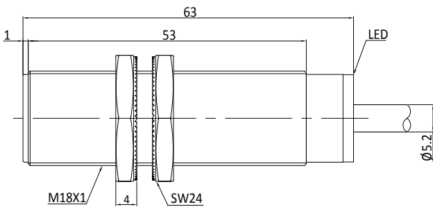
Fig. 3 Inductive sensor with cable (flush)
