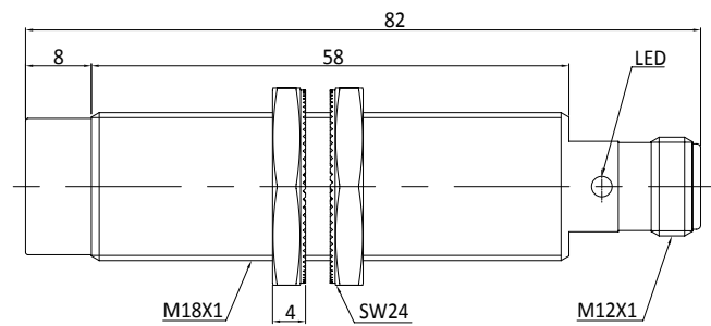
Fig. 10 Inductive sensor with M12 connector (non-flush)
