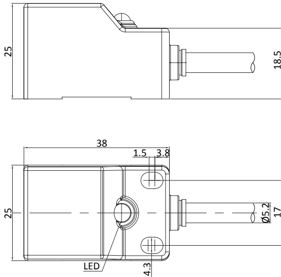
Fig. 1 Inductive sensor with cable (flush/non-flush)
