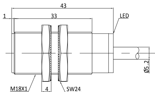
Fig. 1 Inductive sensor with cable (flush)
