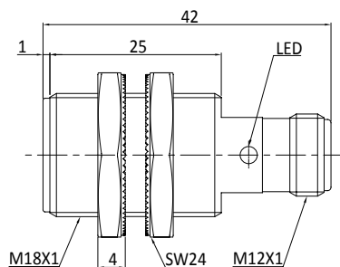
Fig. 3 Inductive sensor with M12 connector (flush)
