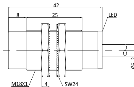
Fig. 2 Inductive sensor with cable (non-flush)
