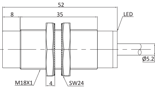
Fig. 5 Inductive sensor with cable (non-flush)
